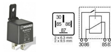
MR26/RELES/POTENCIA
